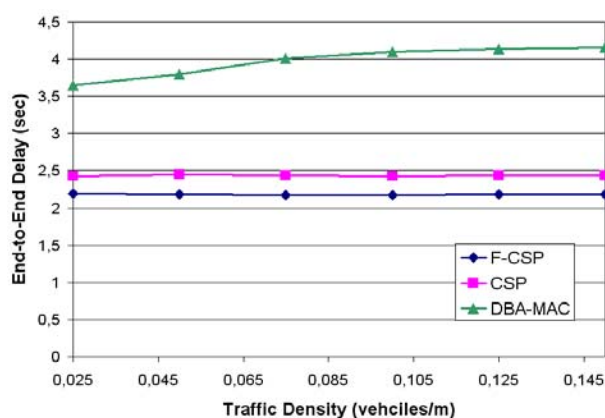
Figure 17. End-to-end delay vs. Traffic density
