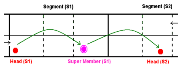
Figure 7. Super member function
