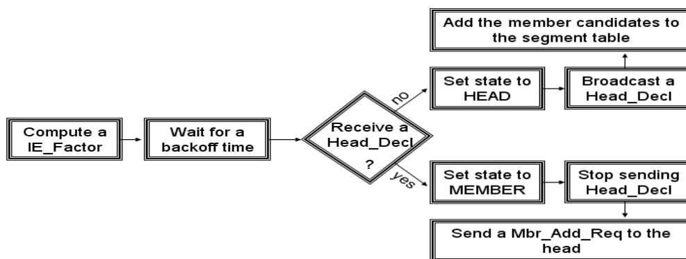
Figure 4. Initial head election process
