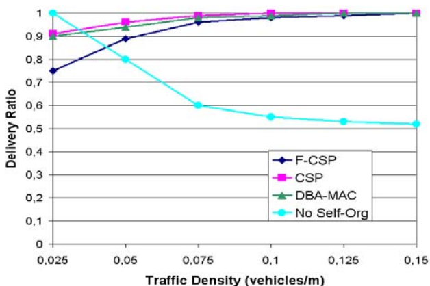
Figure 16. Delivery ratio vs. Traffic density
