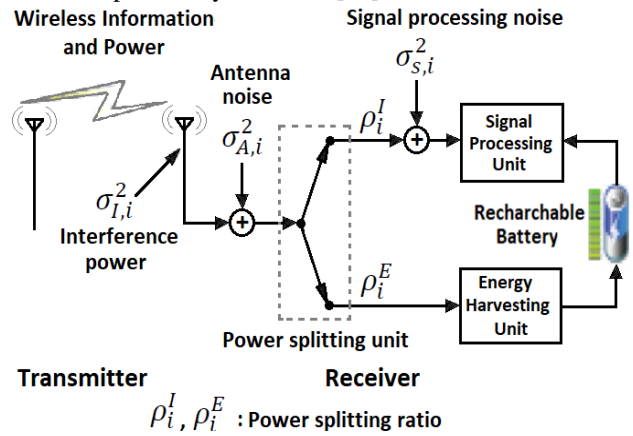
Fig. 2. Model of a receiver with SWIPT.
