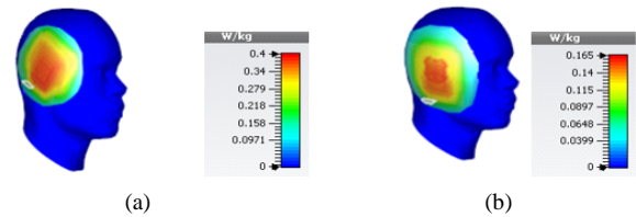
Fig. 12. Specific absorbing rate (SAR) for SPA with 0 iteration, (a) 1g, (b) 10g
