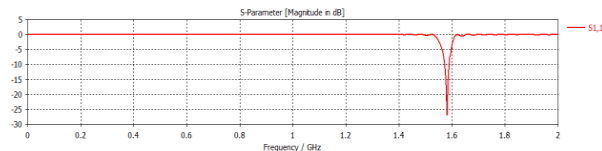
Fig. 10. 3rd iteration Reflection coefficient at 1.575 GHz
