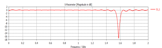
Fig. 4. 0th iteration Reflection coefficient at 1.575 GHz
