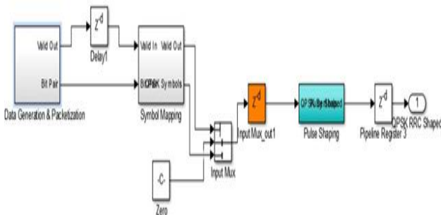
Fig. 2. Connection diagram of internal components of QPSK transmitter subsystem
