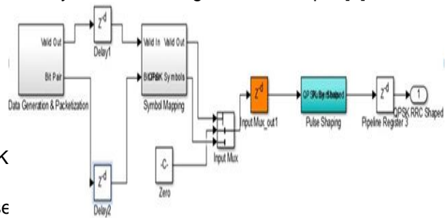
Fig. 3. Connection diagram of internal components of OQPSK transmitter subsystem
