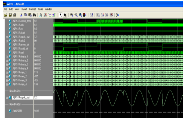
Fig. 7. Simulation for proposed QPSK based modulator
