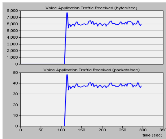
Fig. 6. The rate of receiving voice data traffic scenario 2
