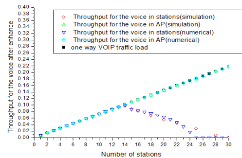
Fig. 15. The capacity after applying our algorithm
