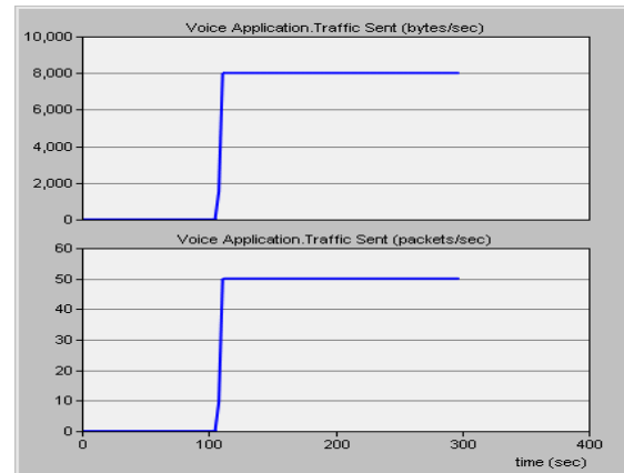
Fig. 3. The rate of sending voice data traffic in scenario 1
