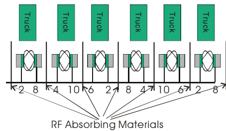
Figure 9. Use of RF absorbing materials. The antennas facing each other at the same door is at least 4 channels away.
