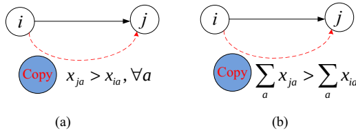
Fig. 2. Single copy multicast in DTNs.
