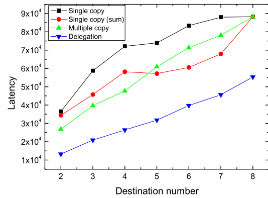
(a) Latency in Intel
