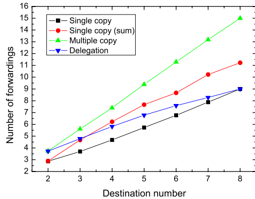
(a) Number of forwardings in Intel
