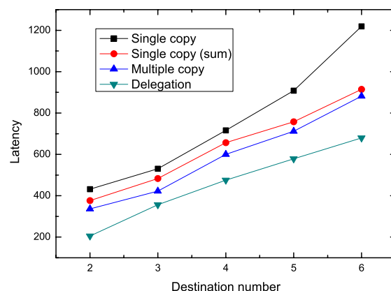
(a) Latency in 20-node trace
