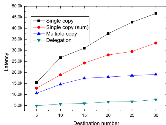
(b) Latency in 100-node trace
