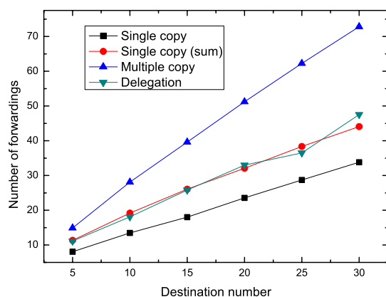
(b) Number of forwardings in 100-node trace
