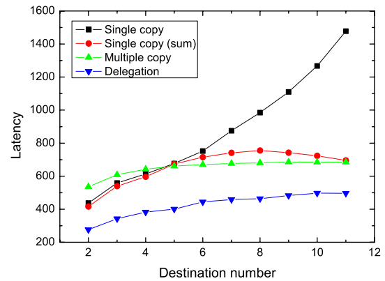
(b) Latency in Cambridge
