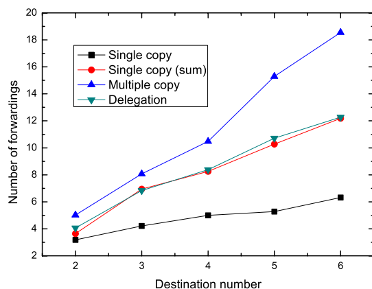
(a) Number of forwardings in 20-node trace
