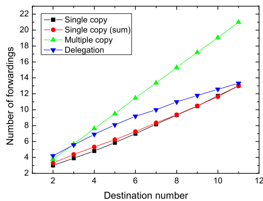
(b) Number of forwardings in Cambridge
