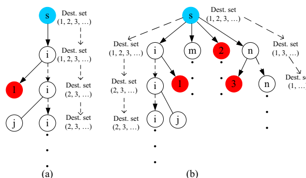
Fig. 1. Multicast tree: (a) single copy; (b) multiple copy and delegation forwarding.
