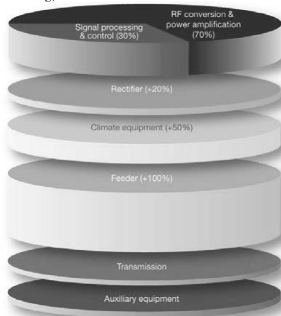
Figure 1. Energy consumption at a typical macro BS (normalized) [6].
