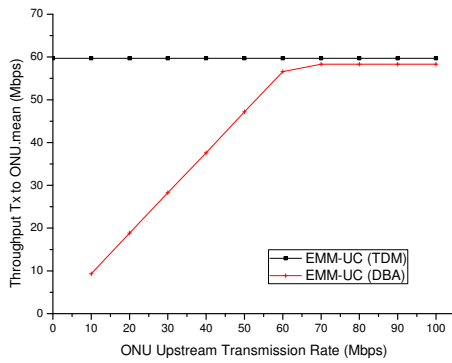
Figure 12. Network throughput compared in different upstream bandwidth allocation schemes.
