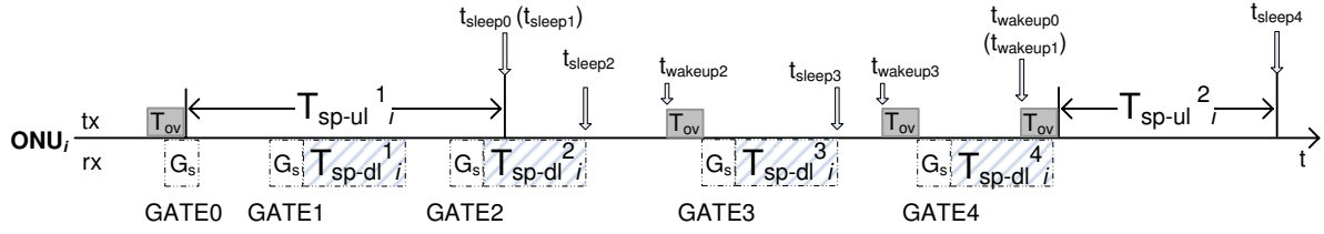
Figure 6. Downstream transmission in the sleep period model.
